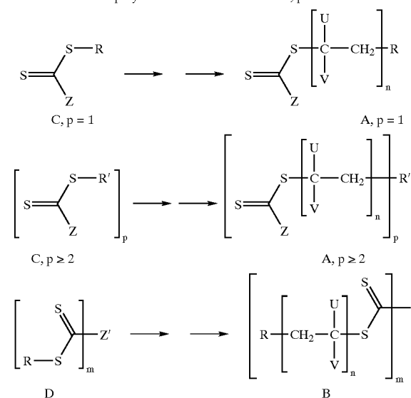
Scheme 4: Formation of linear polymer from CTA of formula C, p = 1
