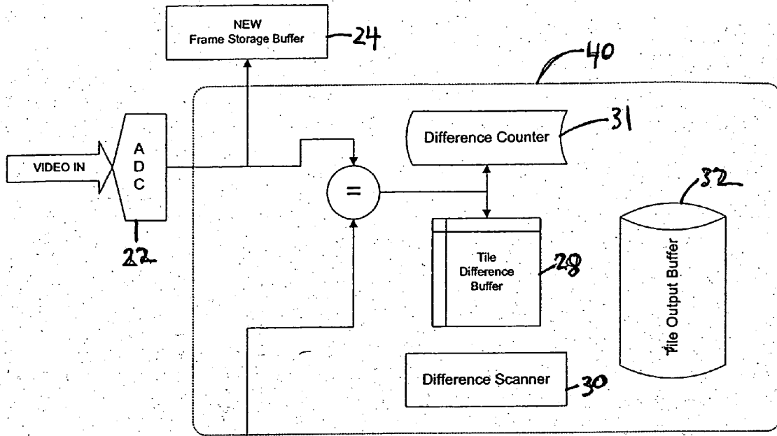
REFERENCE Frame Storage Buffer 26 FPGA in Capture Mode Fig 4A
