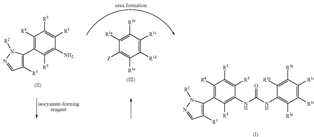
Scheme Ia
