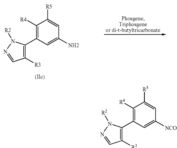
Scheme IIc
