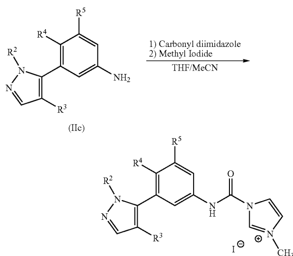
Scheme IIIc
