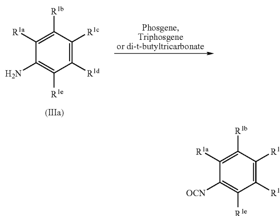
Scheme IIb
