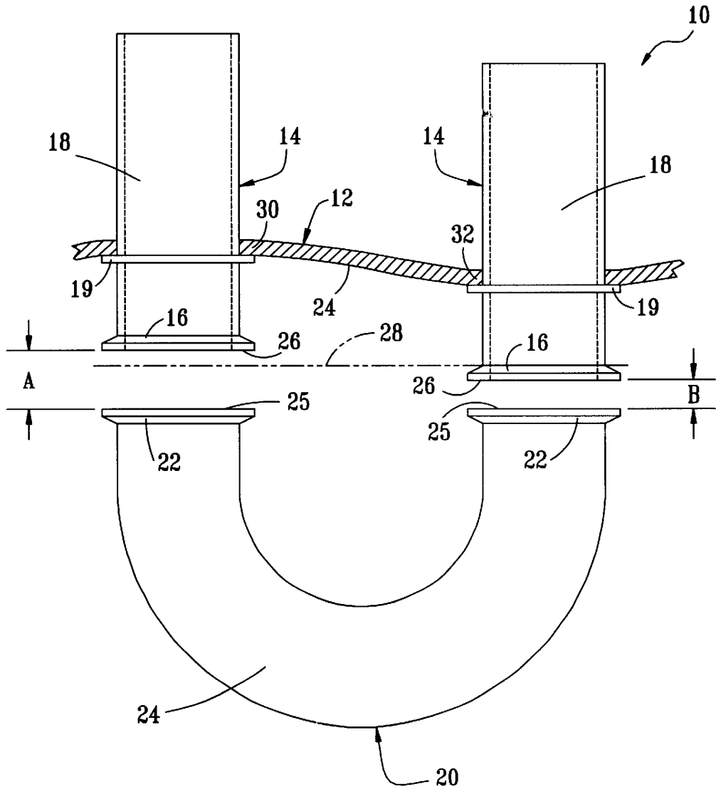
FIG. 1 (Prior Art)
