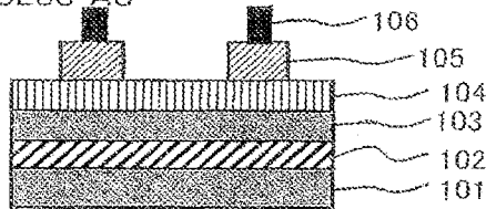
FIG. 26 (Prior Art) PROCESS A3
