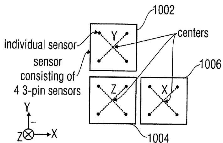
FIGURE 10 (PRIOR ART)
