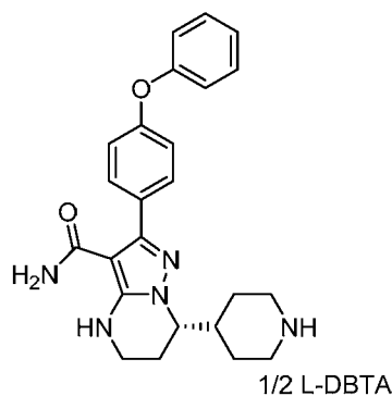
Compound BG-13 .
