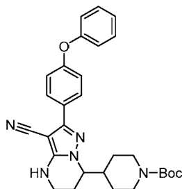
BG-10
