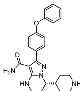
Formula 1f
