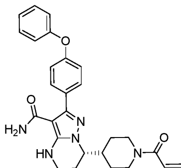
Compound 1
