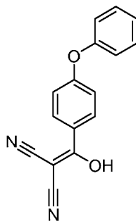
BG-2
