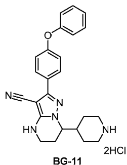
BG-11
