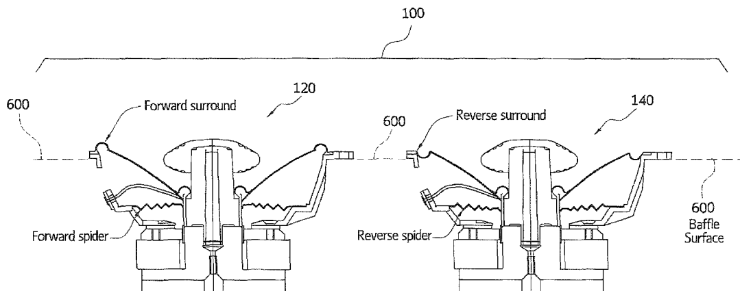
Complementary pair of asymmetrical midrange transducers
