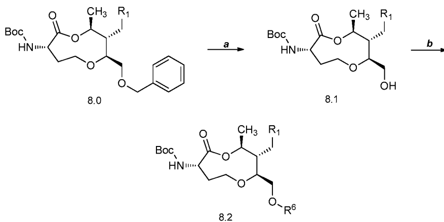
Scheme 8
