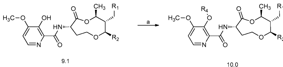
Scheme 10
