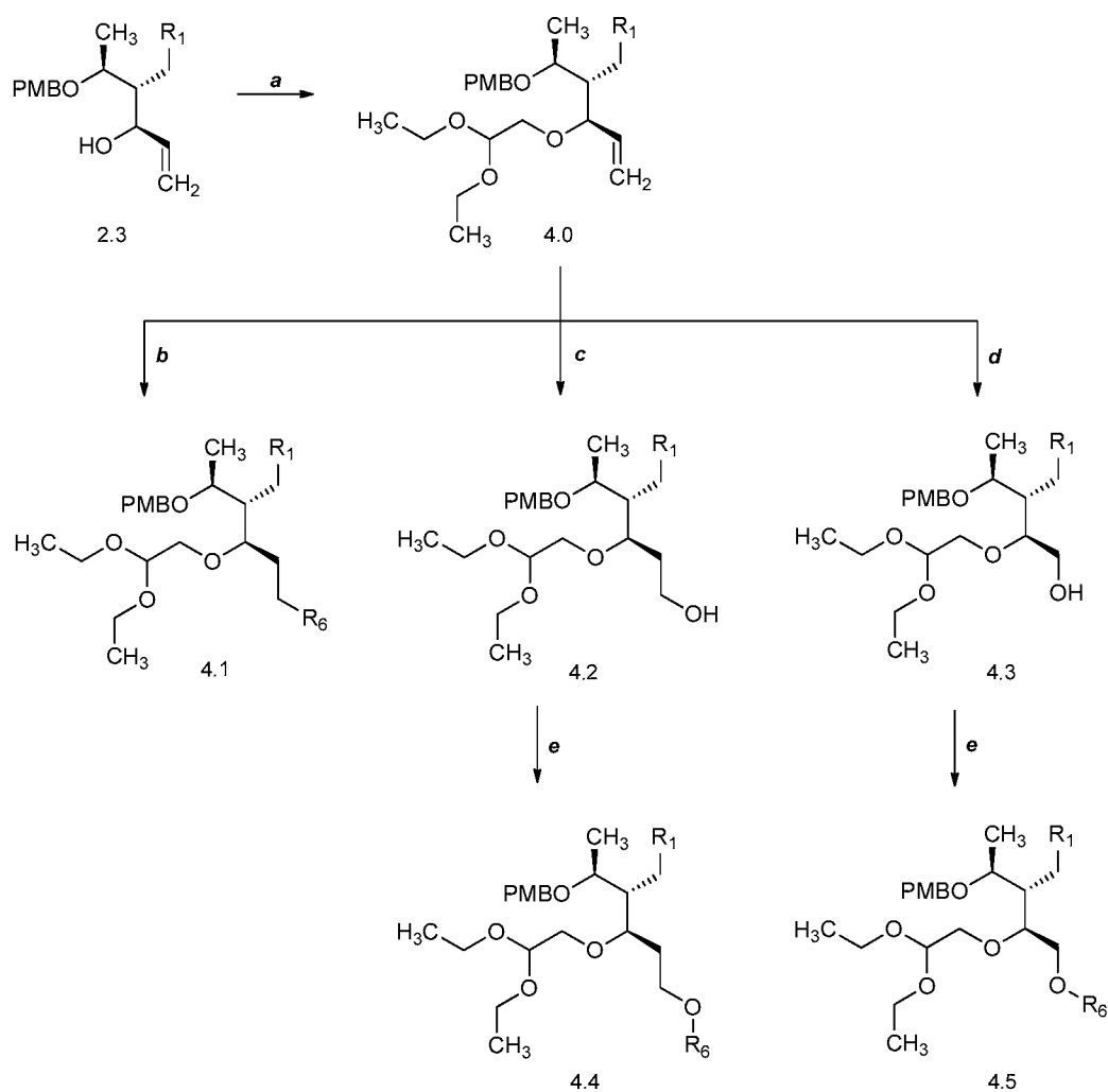
Scheme 4
