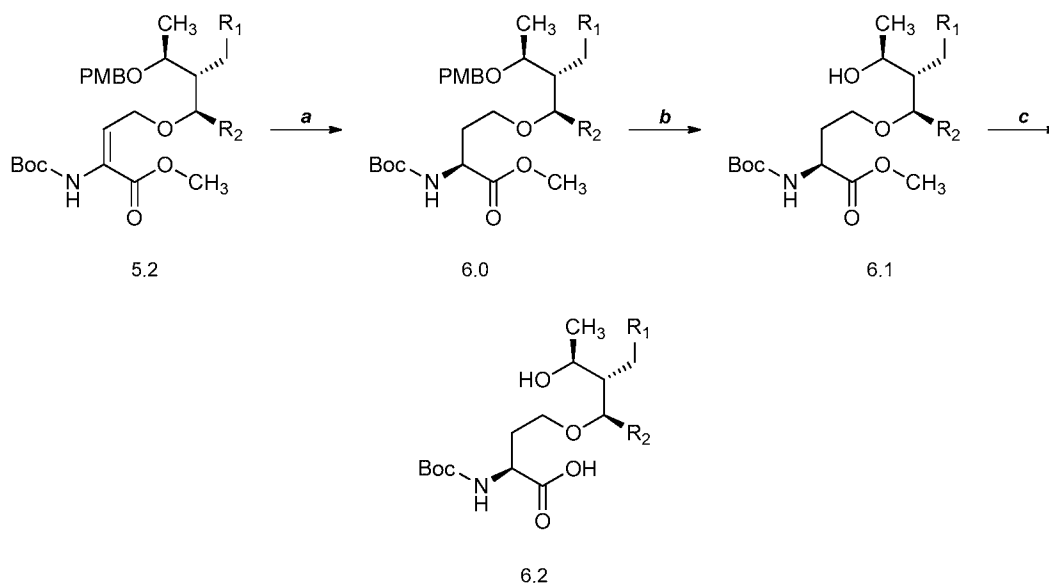
Scheme 6
