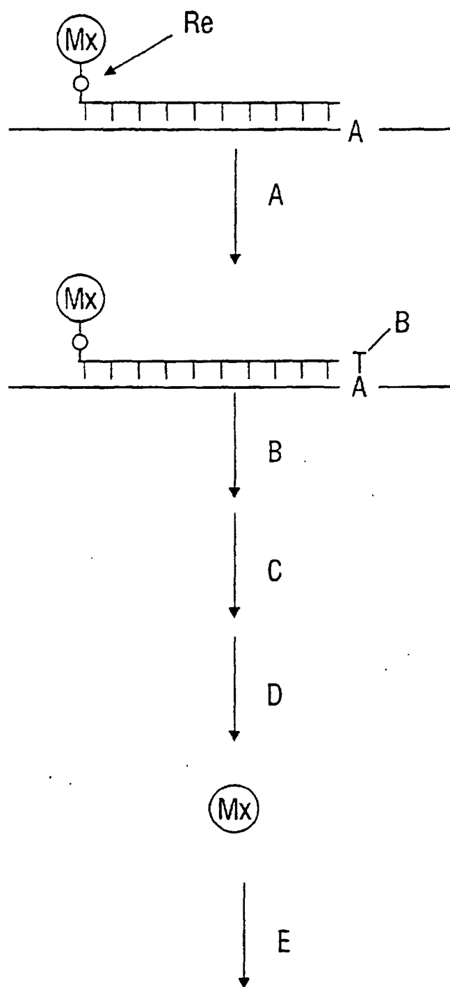
Mass Spec FIG. 2C
