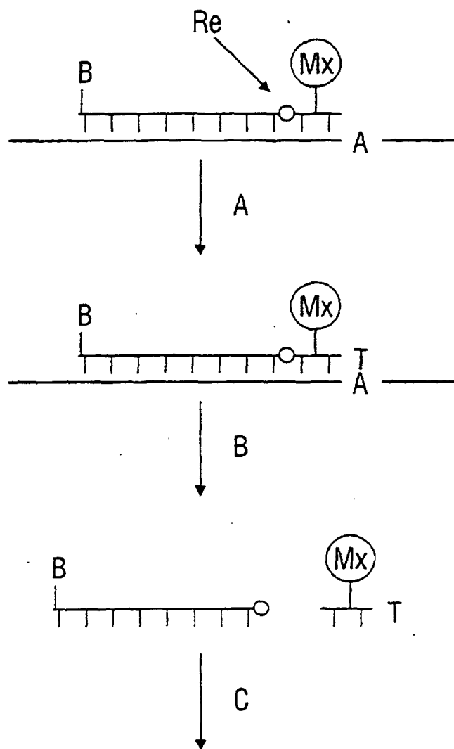
Mass Spec FIG. 2B
