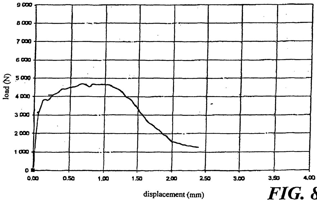
load-displacement diagram
