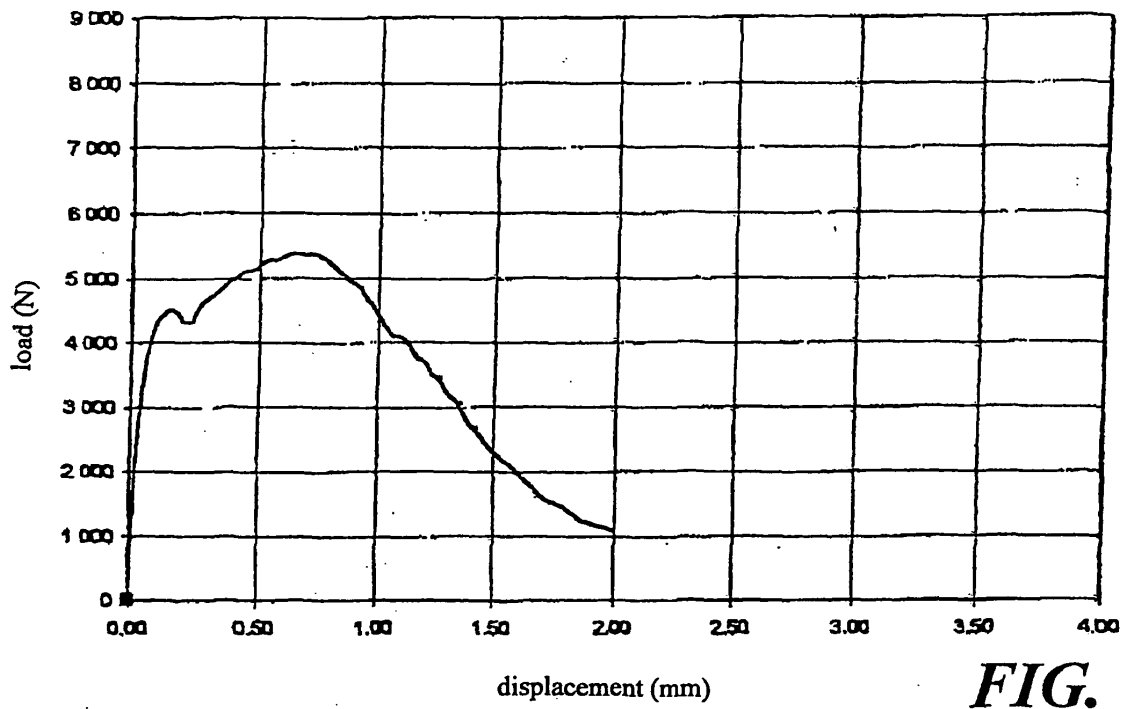
load-displacement diagram
