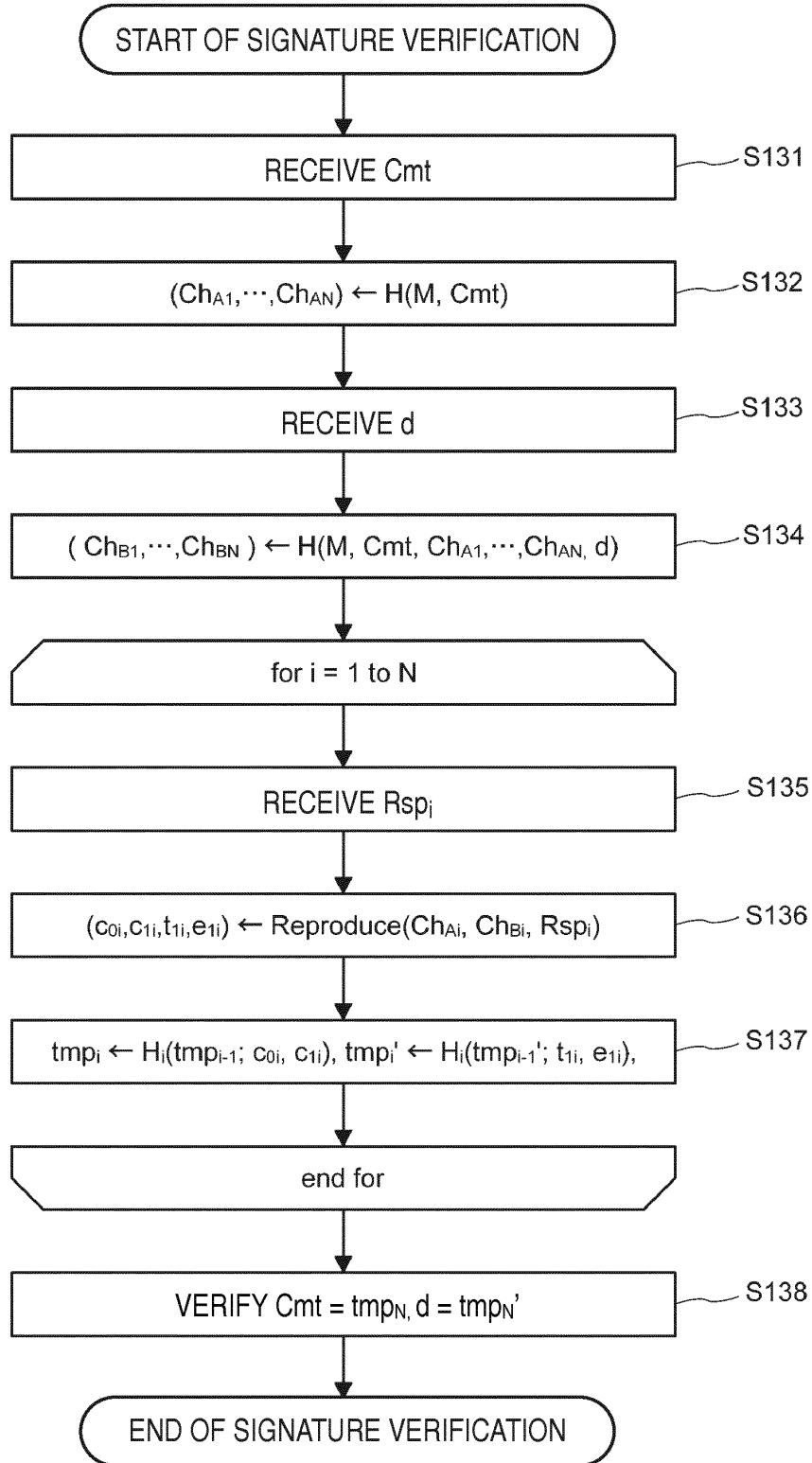
FIG. 14 MEMORY REDUCTION METHOD (DIGITAL SIGNATURE SCHEME BASED ON 5-PASS SCHEME)
