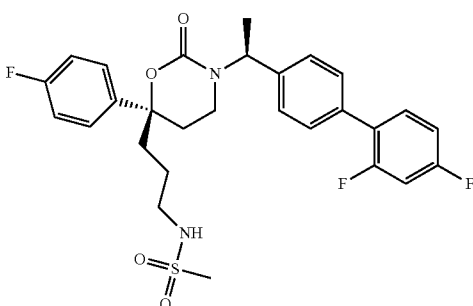
Comparator 10
