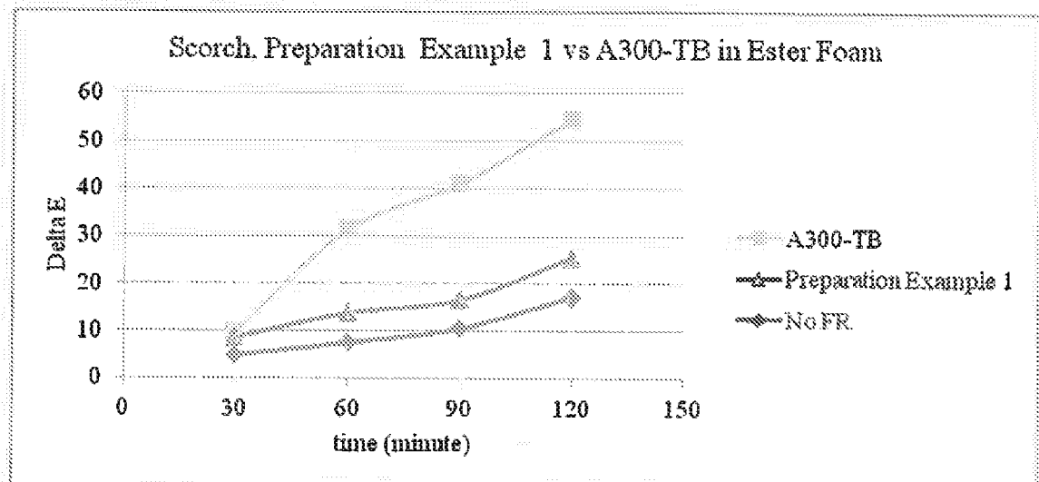
Figure 2. Polyester foam scorch evaluation results
