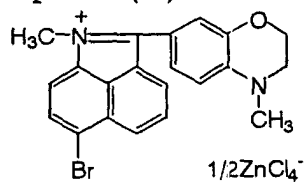
Compound (i)
