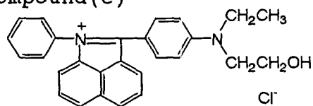
Compound (e)
