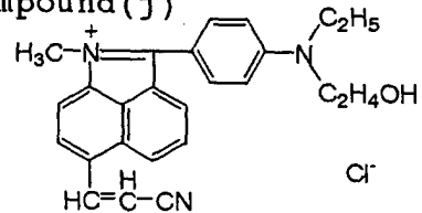
Compound (j)
