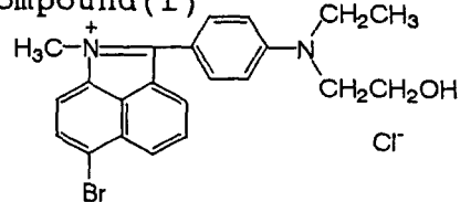
Compound (f)
