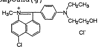
Compound (g)
