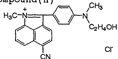
Compound (h)
