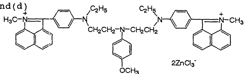
Compound (e)
