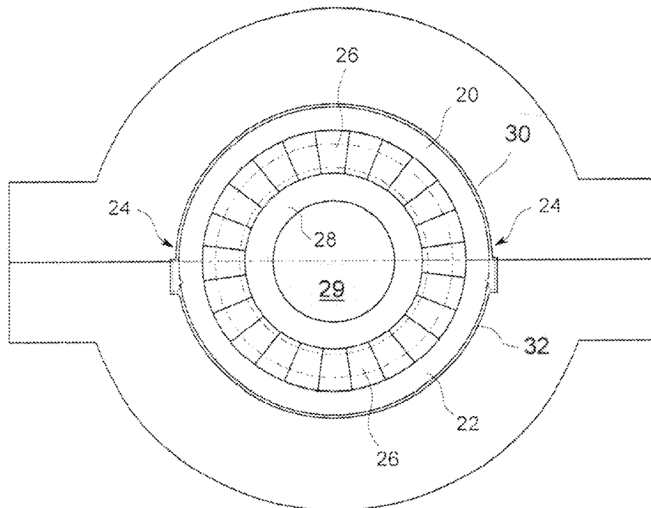
FIG. 2(PRIOR ART)
