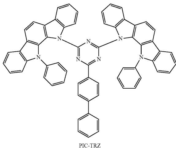
[Chemical Formula 2]
