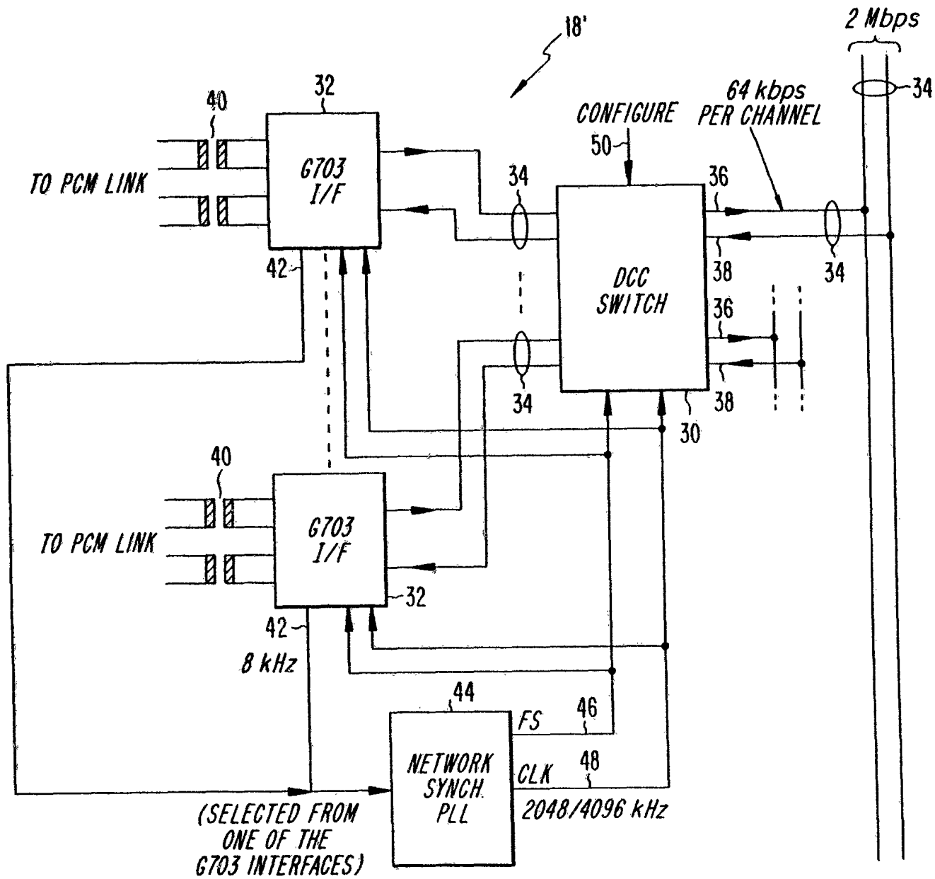
Fig. 1C (PRIOR ART)
