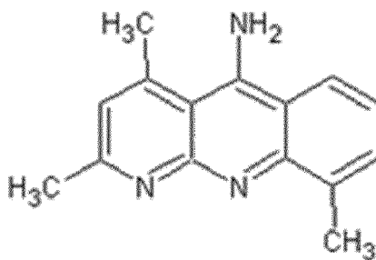
2,4,7,9-tetramethylbenzo[b]-1,8-naphthyridin-5-amine
