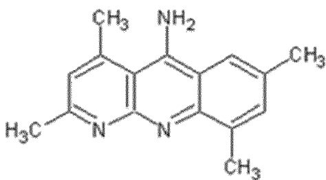
2,4,7,9-tetramethylbenzo[b]-1,8-naphthyridin-5-amine
