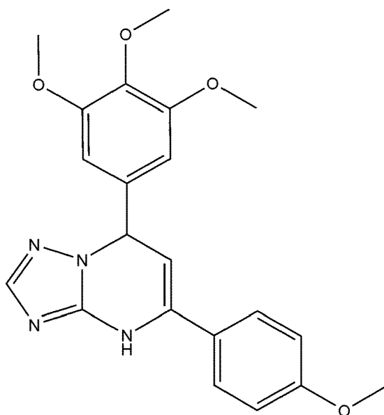
5-(4-ethoxyphenyl)-7-(3,4,5-trimethoxyphenyl)-4,7-dihydro-[1,2,4]triazolo[1,5-a]pyrimidine
