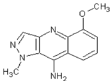
5-methoxy-1-methyl-1H-pyrazolo[4,3-b]quinolin-9-amine
