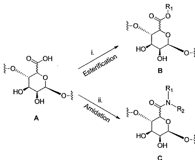
Scheme 1. Representative Reaction Conditions: i. HO-R 1 , 2-Chloro-4,6-dimethoxy-1,3,5-triazine (CDMT), N-methyl morpholine (NMM); ii. HNR 1 R 2 , CDMT, NMM.
