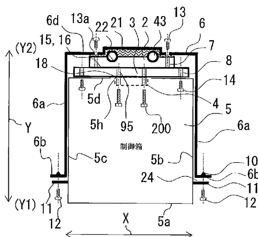
5 Control box
