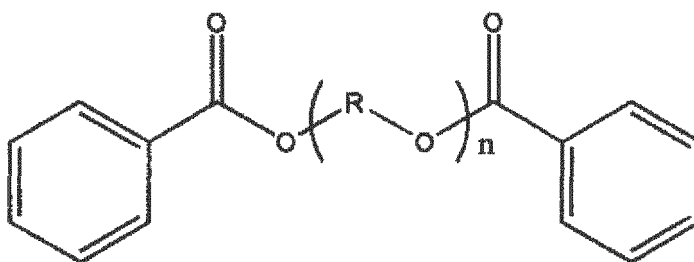
[Chemical Formula 2]
