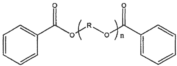
[Chemical Formula 2]
