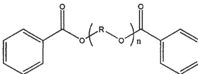
[Chemical Formula 2]
