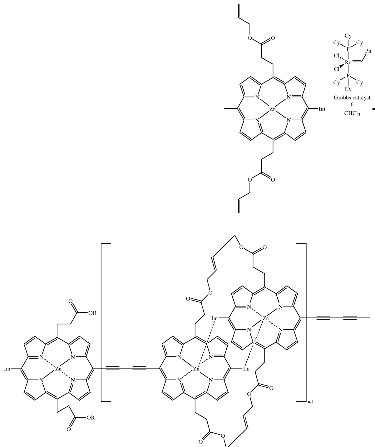
8 One-dimensional coordinated array fixed with covalent bonds
