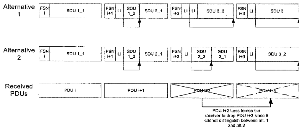
Figure 8 - Error propagation in UMTS R99
