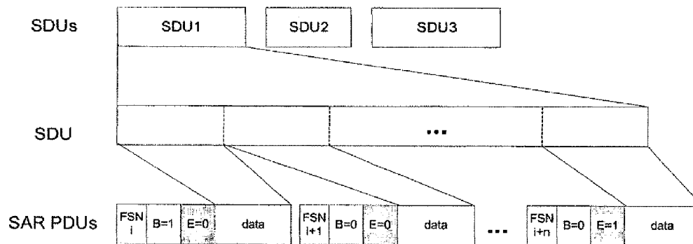
Figure 4 - SAR signaling with Beginning and End flags
