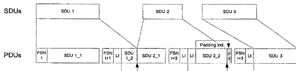
Figure 5 - SAR signaling with length indicators
