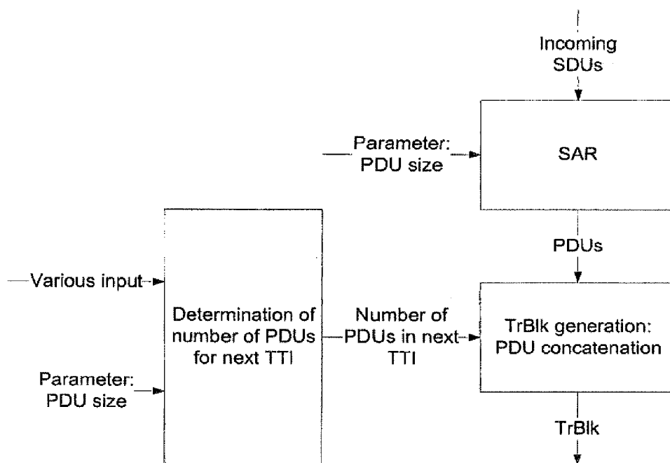
Figure 6 - SDU Segmentation and PDU concatenation Processes
