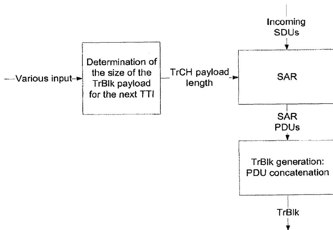
Figure 9 - Proposed SAR and concatenation processes
