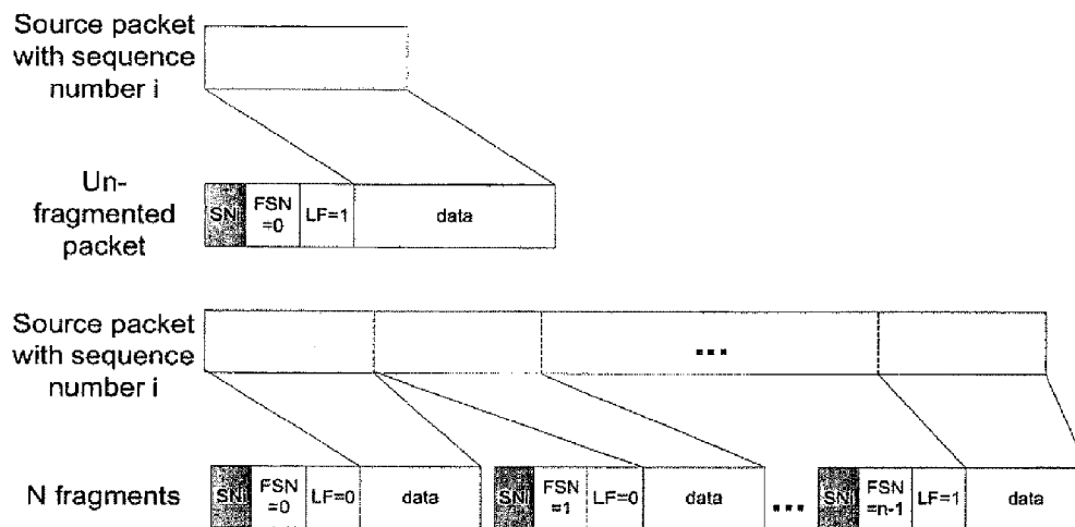
Figure 3 - SAR signaling by fragment numbering
