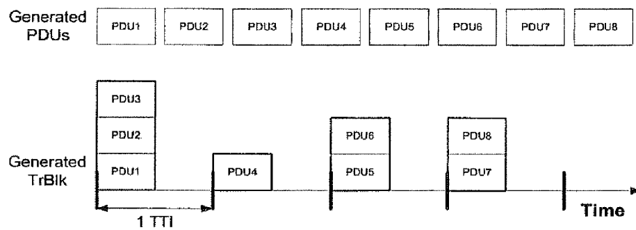
Figure 7 - Transport Channel Block generation
