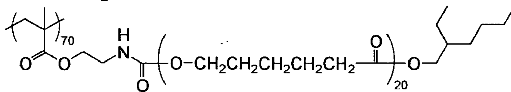
(B-1-2) Mw 32,000
