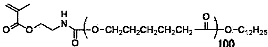
Macromonomer (2-7)
