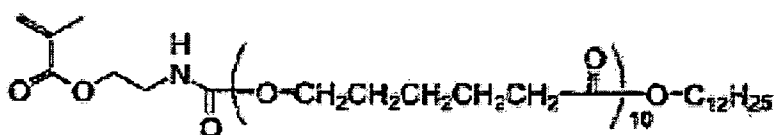
Macromonomer (2-1)
