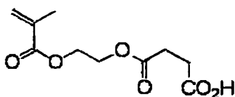
Monomer f
