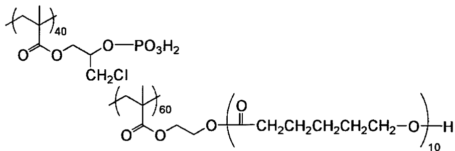
(B-1-4) Mw 28,000
