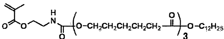
Macromonomer (2-6)
