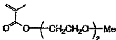
Monomer (2-4)
