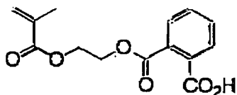
Monomer d
