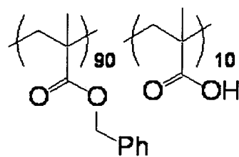
Resin (D-2)
