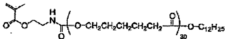
Macromonomer (2-2)
