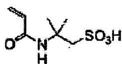
Monomer (2-2)
