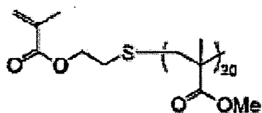
Macromonomer (2-3)
