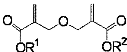
Formula (ED)
