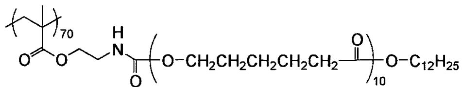
(B-1-1) Mw 13,000
