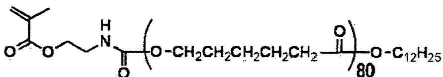
Macromonomer (2-5)
