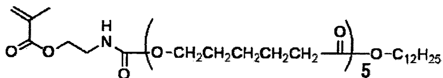
Macromonomer (2-4)
