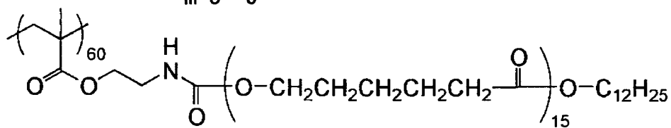
(B-1-3) Mw 28,000
