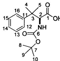
MD021a
