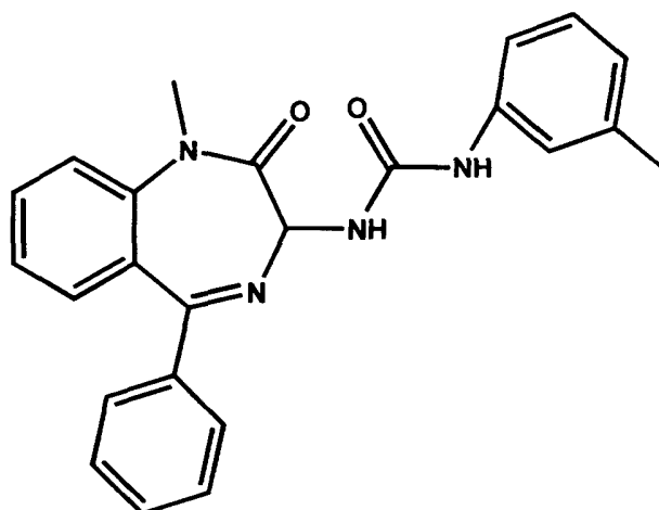
L-365,260
