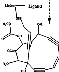
Esperamycin derivatives
