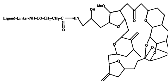
ER-086526 derivatives
