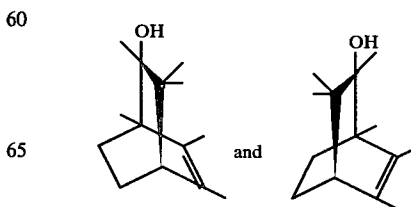
The peaks indicated by reference numerals "901" and "902" are the peaks for the isomers defined according to the structures:
