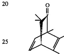
FIG. 5 is the GLC profile for the reaction product of Example II. The peak indicated on FIG. 5 by reference numeral "501" is the peak for the compound having the structure:
