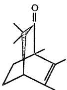
FIG. 8 is the infra-red spectrum for the compound of peak 501 of FIG. 5 having the structure:
