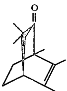
FIG. 9 is the GLC profile for fraction 2 of the distillation product of the reaction product of Example III containing the compounds defined according to the structures:
