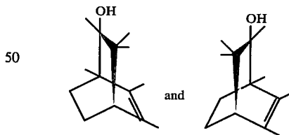
The peaks indicated by reference numerals "901" and "902" are the peaks for the isomers defined according to the structures:
