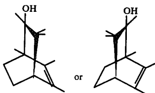
FIG. 13 is the mass spectrum for the peak indicated by reference numeral 902 of FIG. 9 for the compound having the structure:
