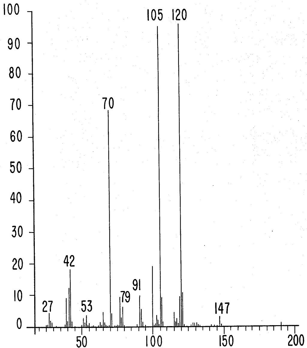
MASS SPECTRUM FOR PEAK 101 OF FIG. 1, EXAMPLE I.
