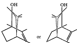
FIG. 13 is the mass spectrum for the peak indicated by reference numeral "902" of FIG. 9 for one of the compounds having the structures:
