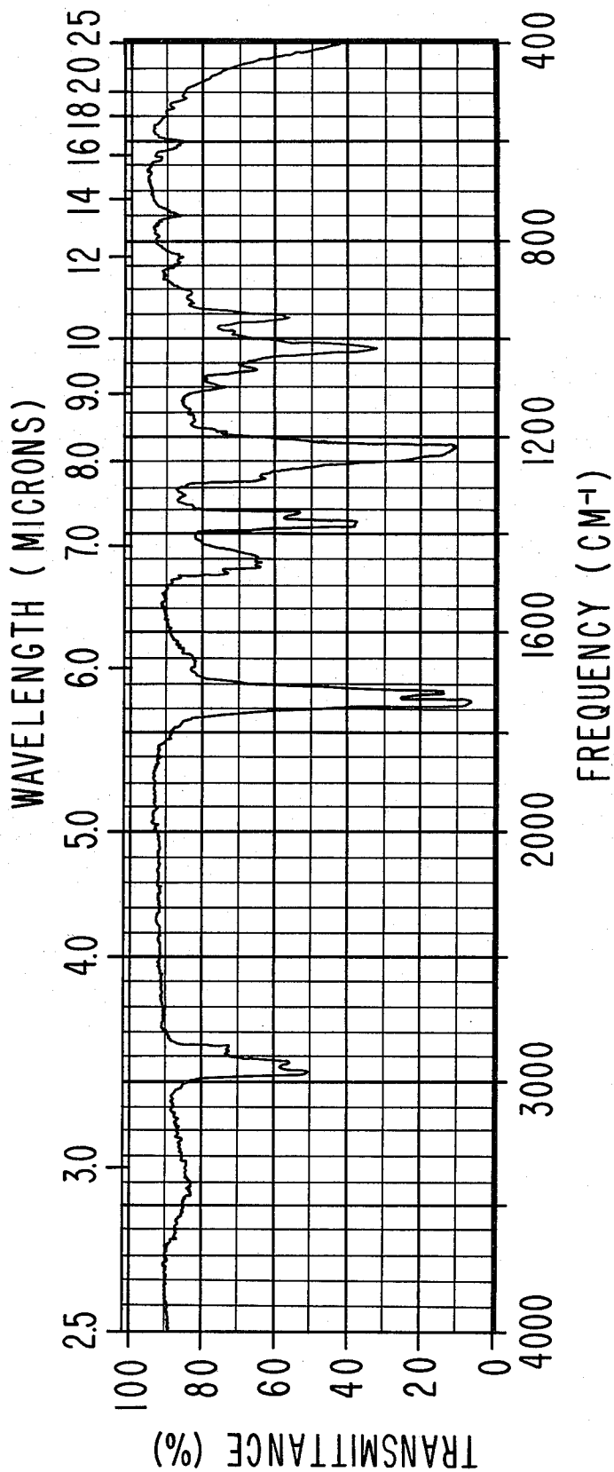
IR SPECTRUM FOR PEAK 201 OF FIG. 20 FOR EXAMPLE V.
