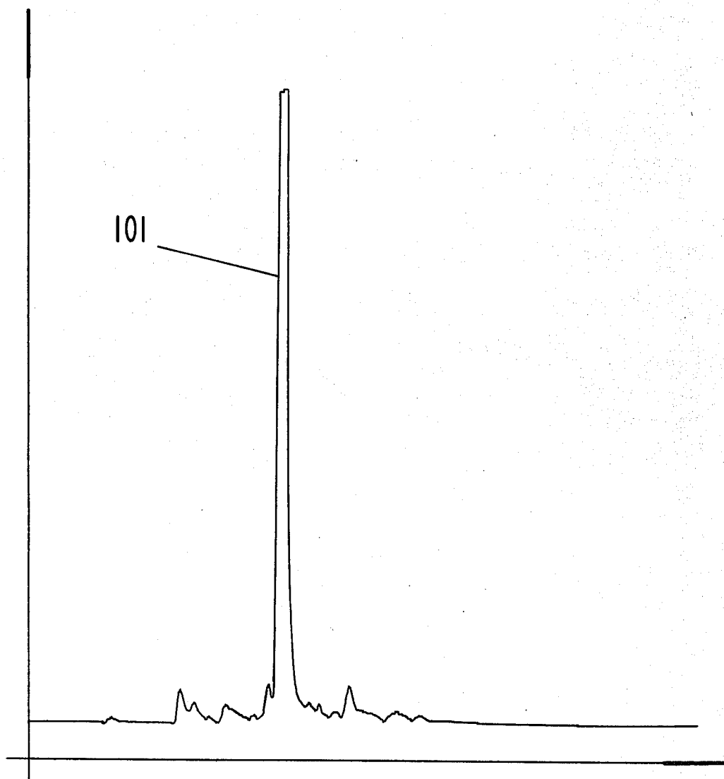
GLC PROFILE FOR EXAMPLE I .
