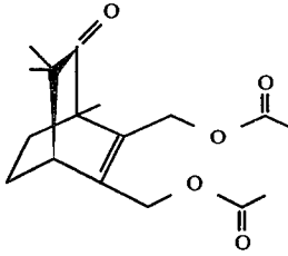
FIG. 24 is the GLC profile for the reaction product of Example VI containing the compound defined according to the structure:
