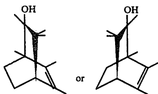
FIG. 15 is the NMR spectrum for the peak indicated by reference numeral "902" of FIG. 9 for one of the compounds produced according to Example III having one of the structures:
