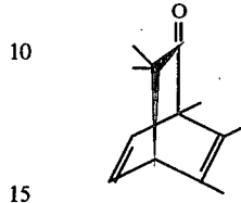
The peak indicated by the reference numeral "101" is for the compound having the structure:
