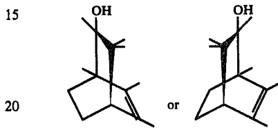
FIG. 15 is the NMR spectrum for the compound of peak 902 of FIG. 9 having the structure:
