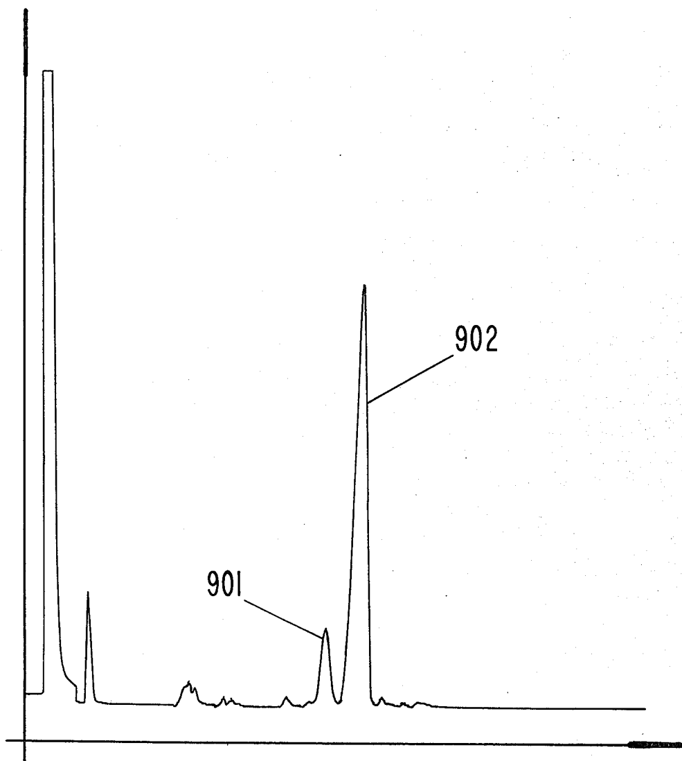
GLC PROFILE FOR EXAMPLE III.
