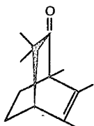
FIG. 6 is the mass spectrum for the compound of peak 501 of FIG. 5 having the structure:
