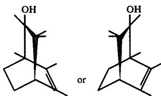
FIG. 14 is the infra-red spectrum for the compound of peak 902 of FIG. 9 having the structure:
