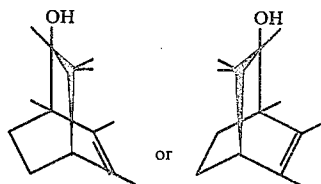
FIG. 11 is the infra-red spectrum for the compound of peak 901 of FIG. 9 having one of the structures:
