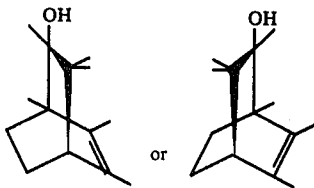
FIG. 11 is the infra-red spectrum for the compound 25 of peak 901 of FIG. 9 having the structure:
