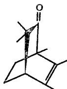
FIG. 7 is the NMR spectrum for the compound of peak 501 of FIG. 5 having the structure:
