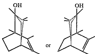
FIG. 12 is the NMR spectrum for the compound of peak 901 of FIG. 9 produced according to Example III containing one of the compounds having the structures:
