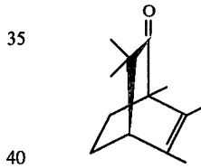
FIG. 9 is the GLC profile for fraction 2 of the distillation product of the reaction product of Example III containing the compounds defined according to the structures:
