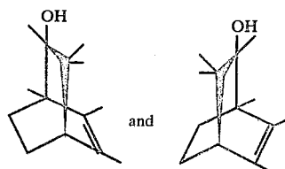
FIG. 10 is the mass spectrum for the peak indicated by reference numeral "901" of FIG. 9 for one of the compounds produced according to Example III having one of the structures:
