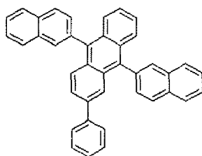
9,10-di(naphthalen-2-yl)-2-phenylantracene (PADN), CAS 865435-20-7, -2.37 V, B4;
