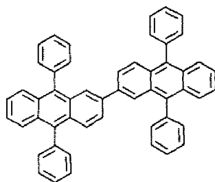
9,9',10,10'-tetraphenyl-2,2'-bianthracene (TPBA), CAS 172285-72-2, -2.28 V, B1;
