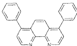
4,7-diphenyl-1,10-phenanthroline (Bphen) CAS 1662-01-7, - 2.47 V, C7;
