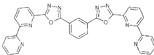
1,3-bis[2-(2,2'-bipyridine-6-yl)-1,3,4-oxadiazol-5-yl]benzene (Bpy-OXD), -2.28 V, C8;
