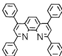
2,4,7,9-tetraphenyl-1,10-phenanthroline, CAS 51786-73-3, -2.33 V, B3;
