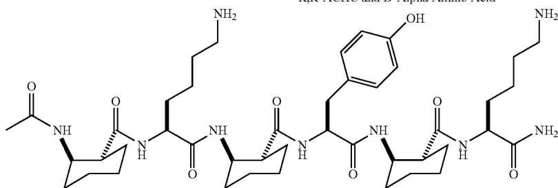
R,R-ACHC and L-Alpha Amino Acid
