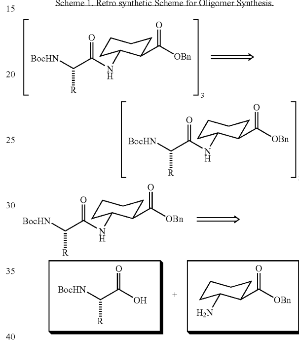
Scheme 1. Retro synthetic Scheme for Oligomer Synthesis.
