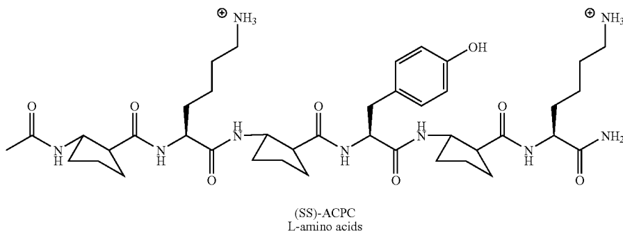
First generation \alpha/\beta peptides
