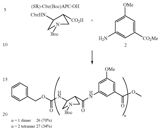
Scheme 9
