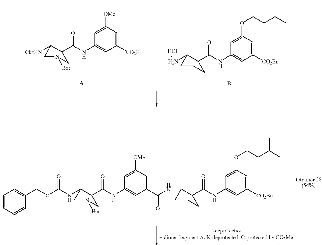
Scheme 10
