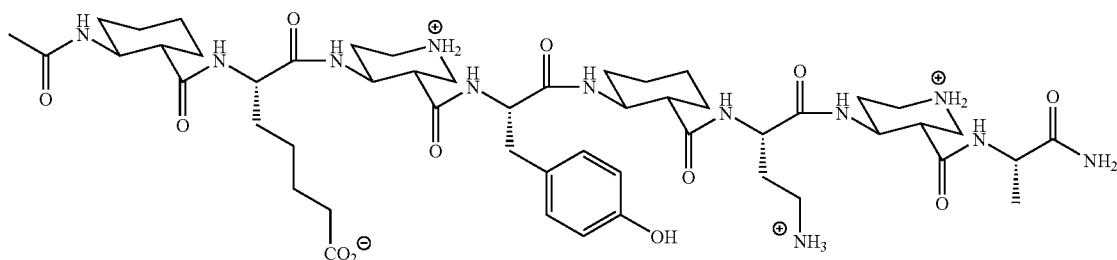
Ac-ACHC-E-PIP-Y-ACHC-K-PIP-A-NH 2 (S) ACHC, (S) PIP, (L) amino acids
