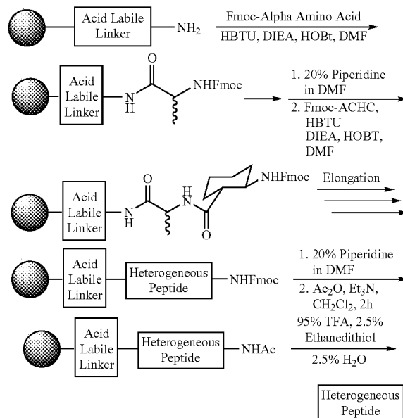
Scheme 3. Generalized Route for Solid Phase Synthesis
