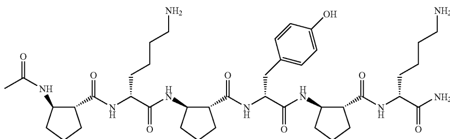
(R,R)-ACPC D-amino acids
