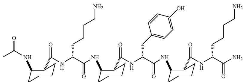
R,R-ACHC and D-Alpha Amino Acid
