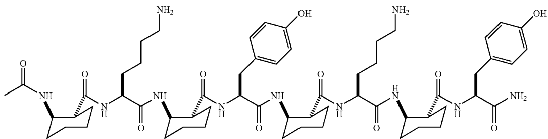
R,R-ACHC and L-Alpha Amino Acid
