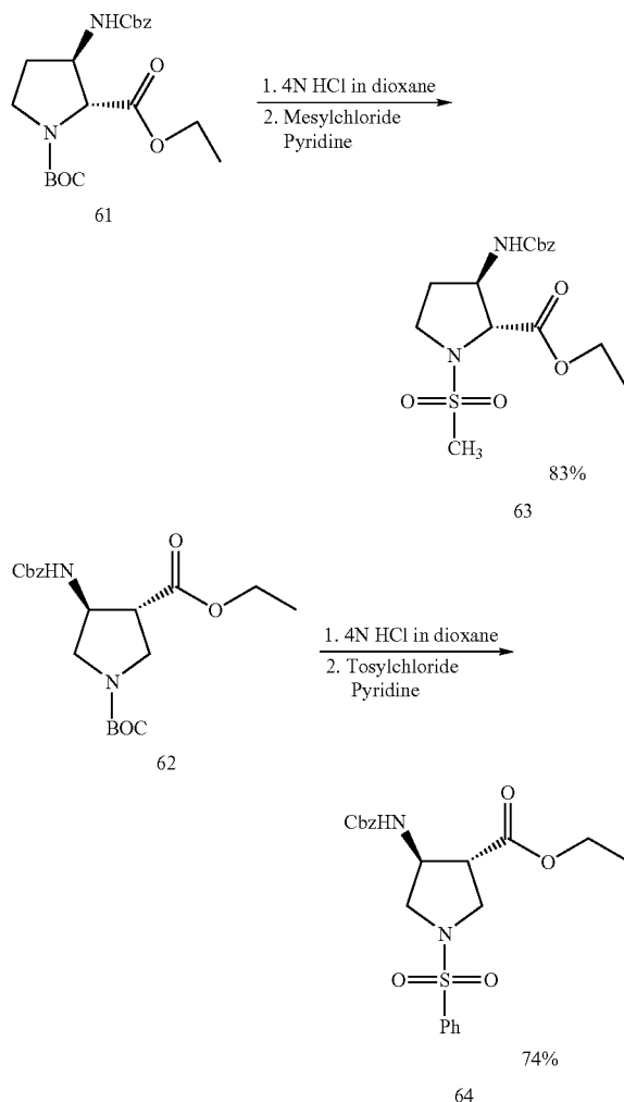
REACTION 10
