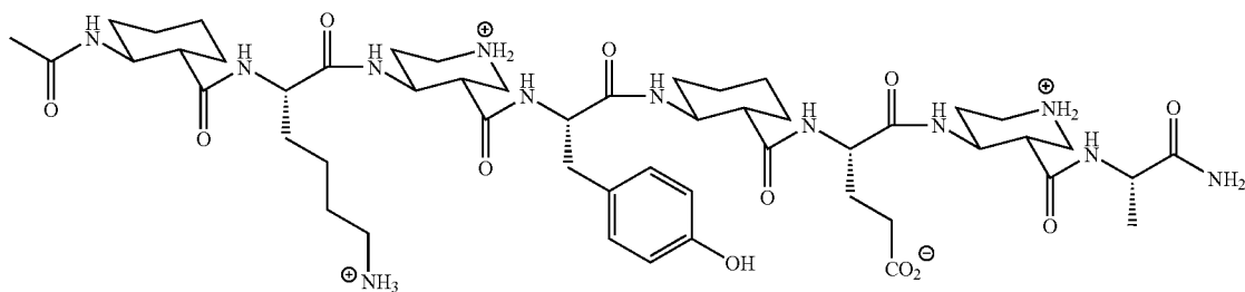
6-ring α/β peptides 43-46
