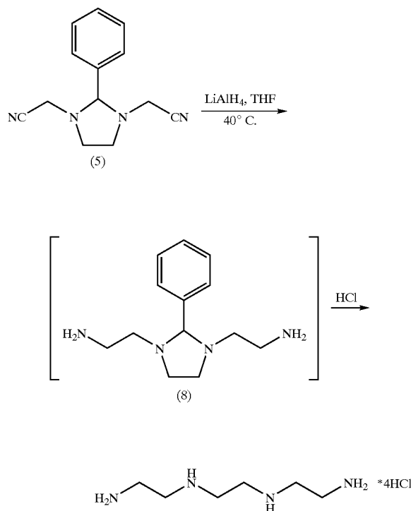
Scheme 9
