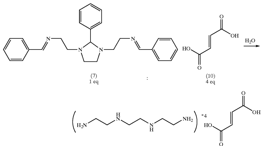
Scheme 7
