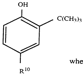
2-t-butyl-4-R 10 -phenol
