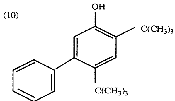
2,4-di-t-butyl-5-phenylphenol
