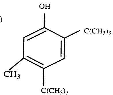
2,4-di-t-butyl-5-methylphenol
