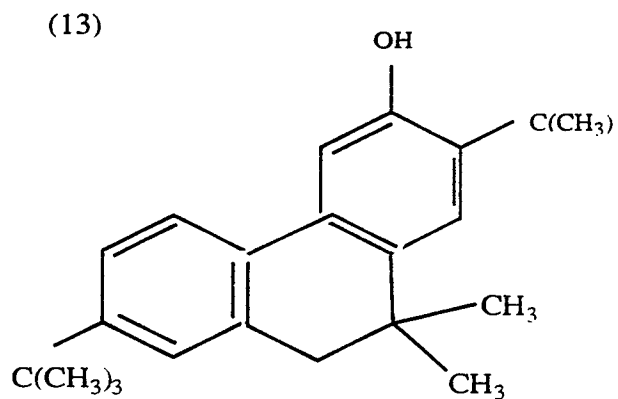
2-t-butyl-3-hydroxy-10,10-dimethyl-9,10-dihydrophenanthrene
