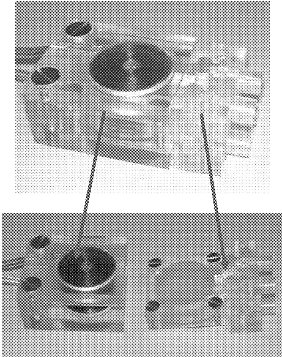
Clam Shell and Micropump—Fully Assembled
