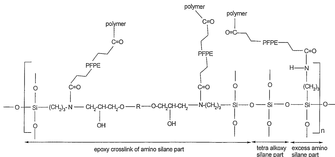
Formula 6
