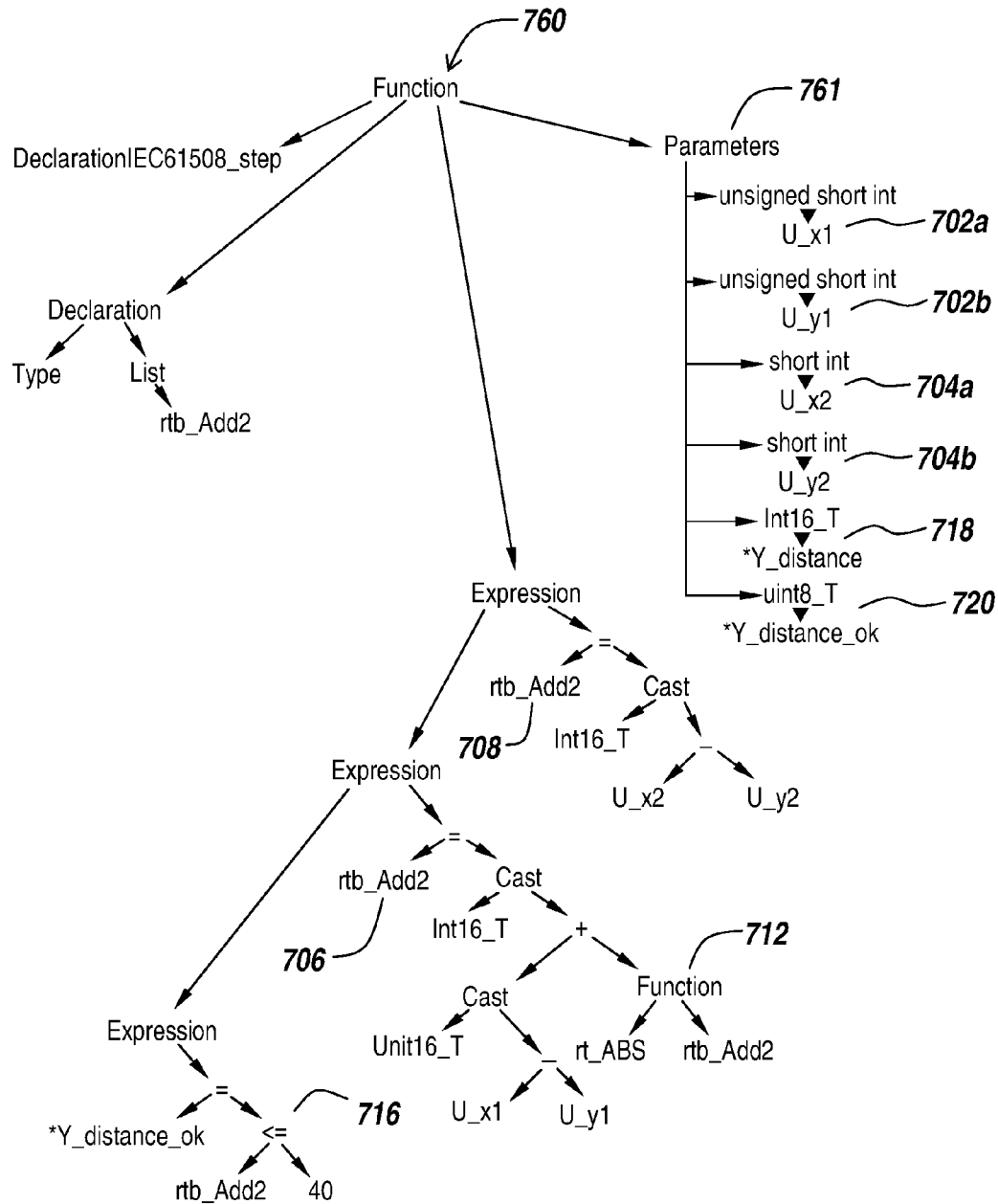
Abstract Syntax Tree (AST)
