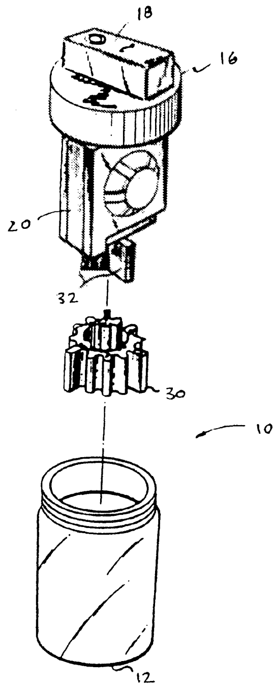
FIG. 4 PRIOR ART
