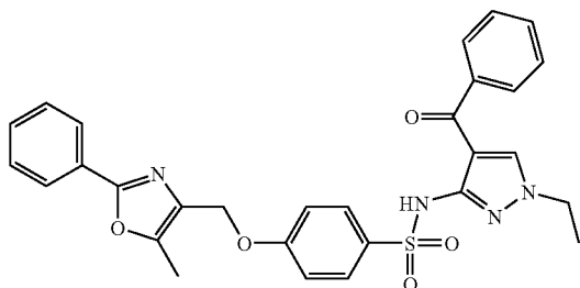
A. (3-Amino-1-ethyl-1H-pyrazol-4-yl)-phenyl-methanone
