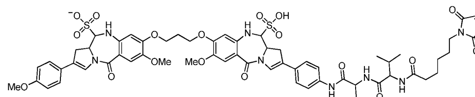
Imine di-sulfo talirine
