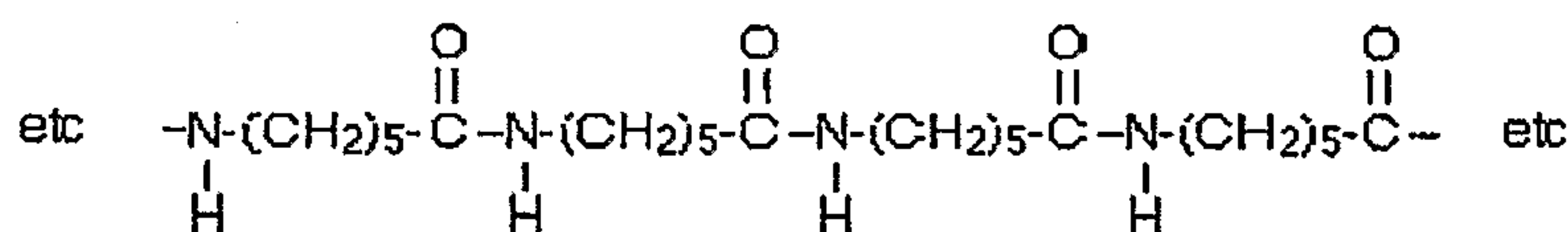
nylon 6
