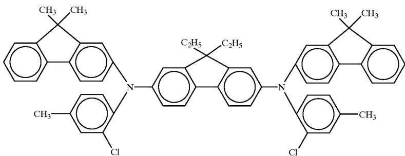
Compound 16
