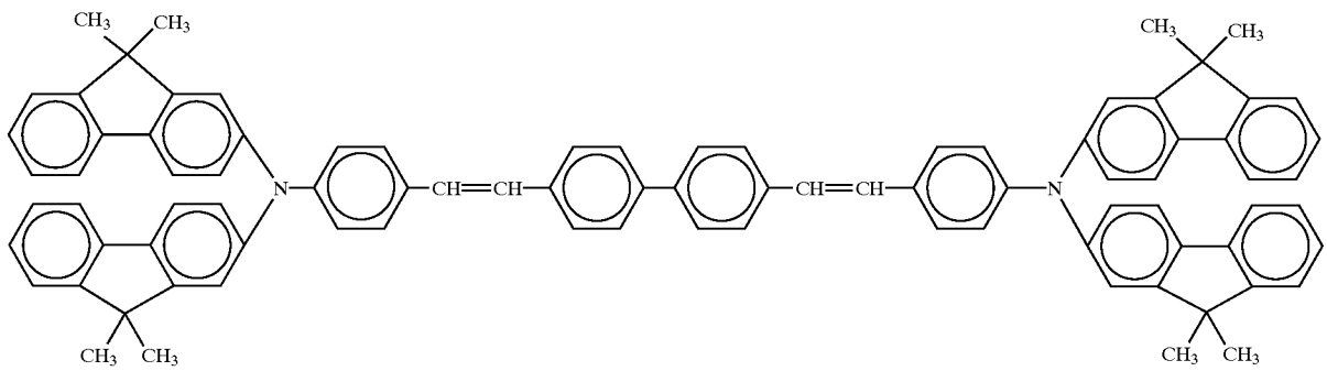
Compound 68
