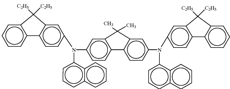
Compound 15
