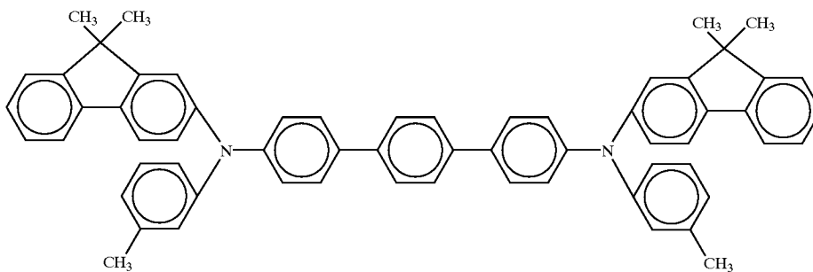
Compound 13
