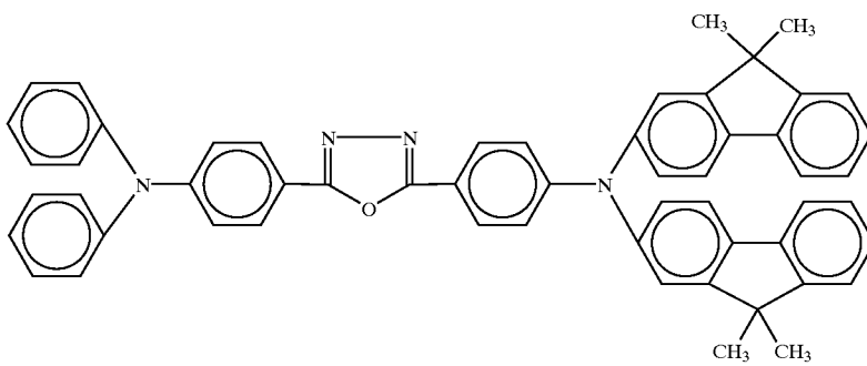
Compound 83
