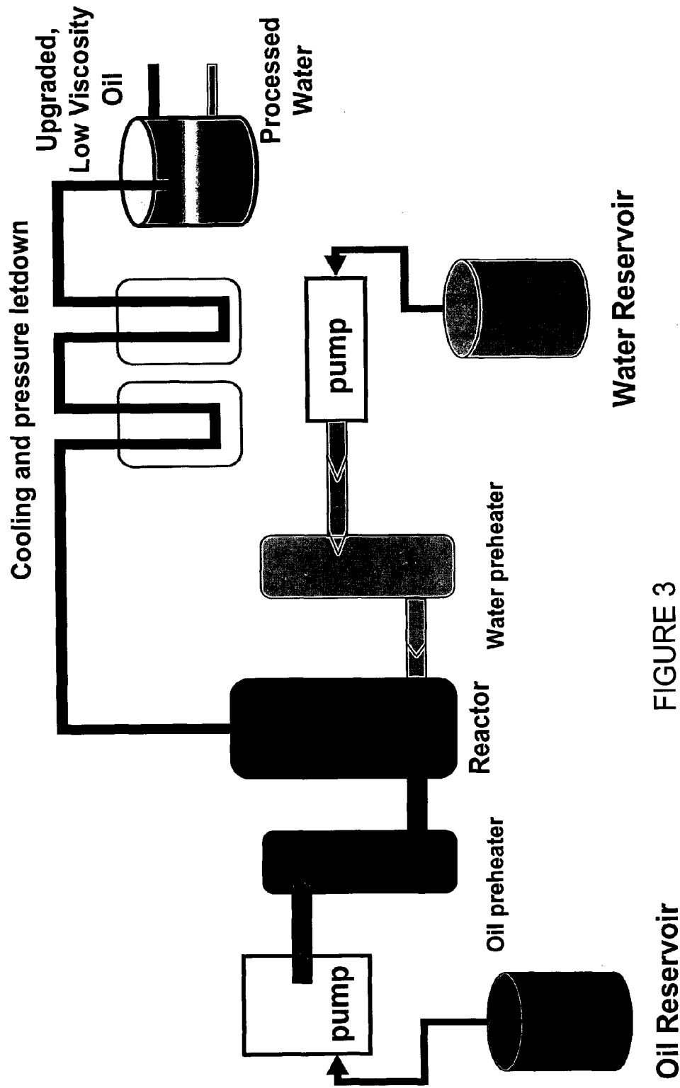
General Flow-Through System with Oil Preheater
