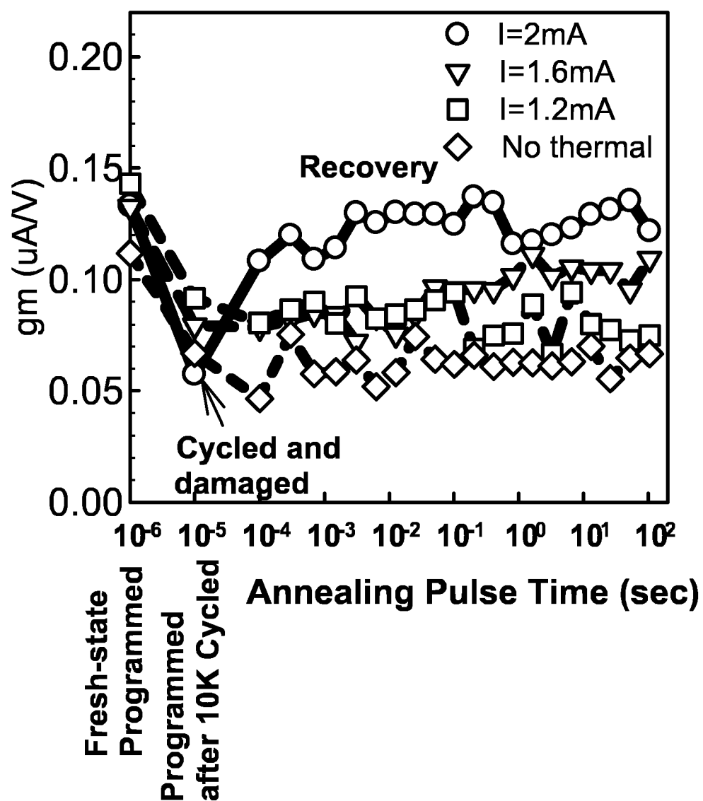
(c) g_m recovery during thermal annealing
