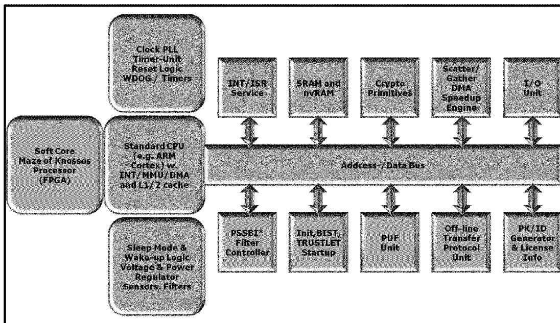
Block diagram of the CASTOR HSM.
