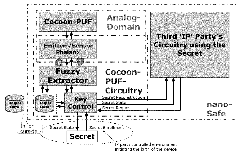
Figure 21: Block Diagram of a CASTOR.
