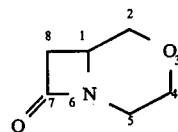
3-oxa-6-aza-bicyclo-[4,2,0]octan-7-one.
