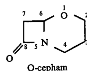
O-cepham
