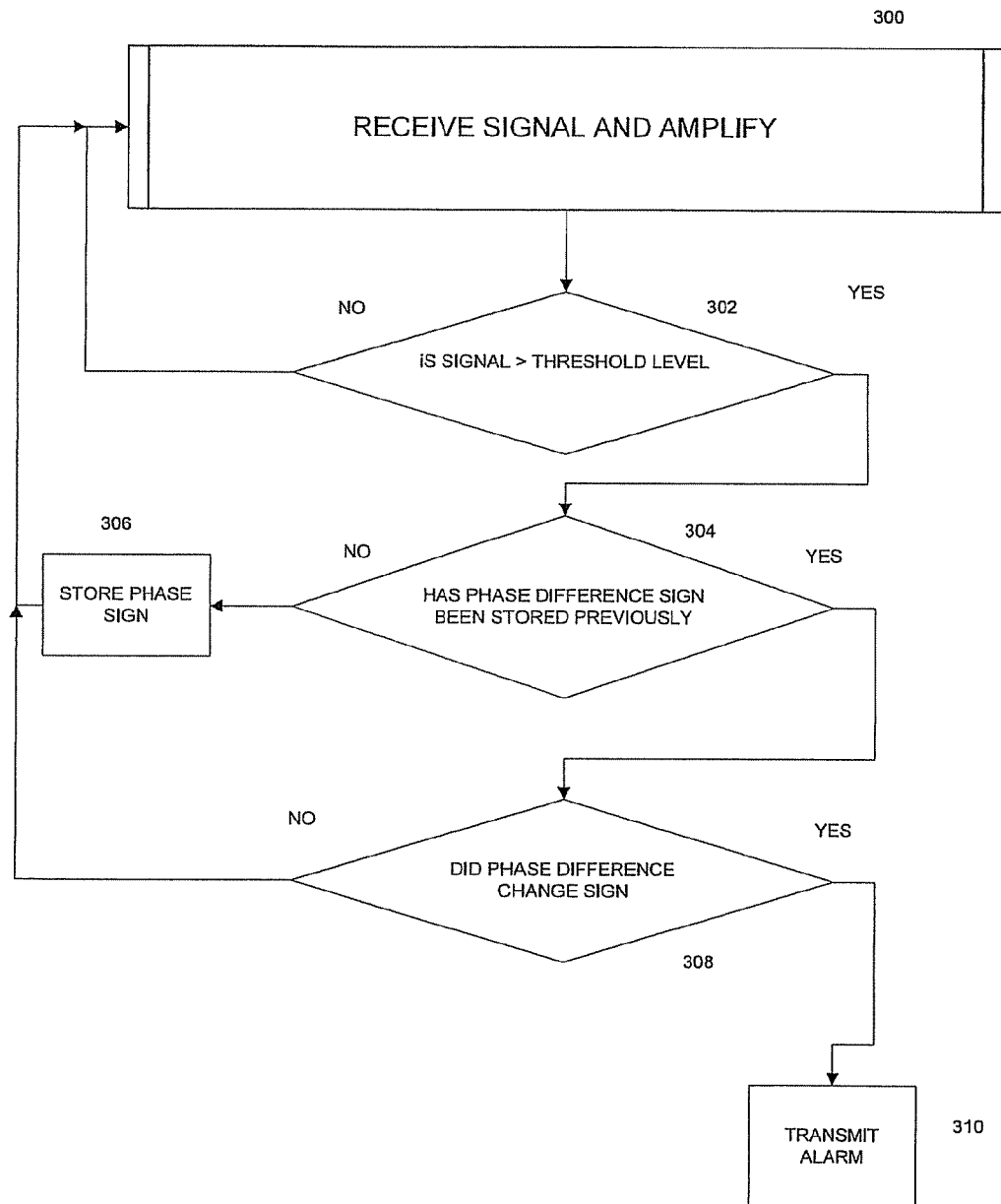
FIGURE 6 - MICROWAVE CURTAIN LENS LOGIC FLOWCHART
