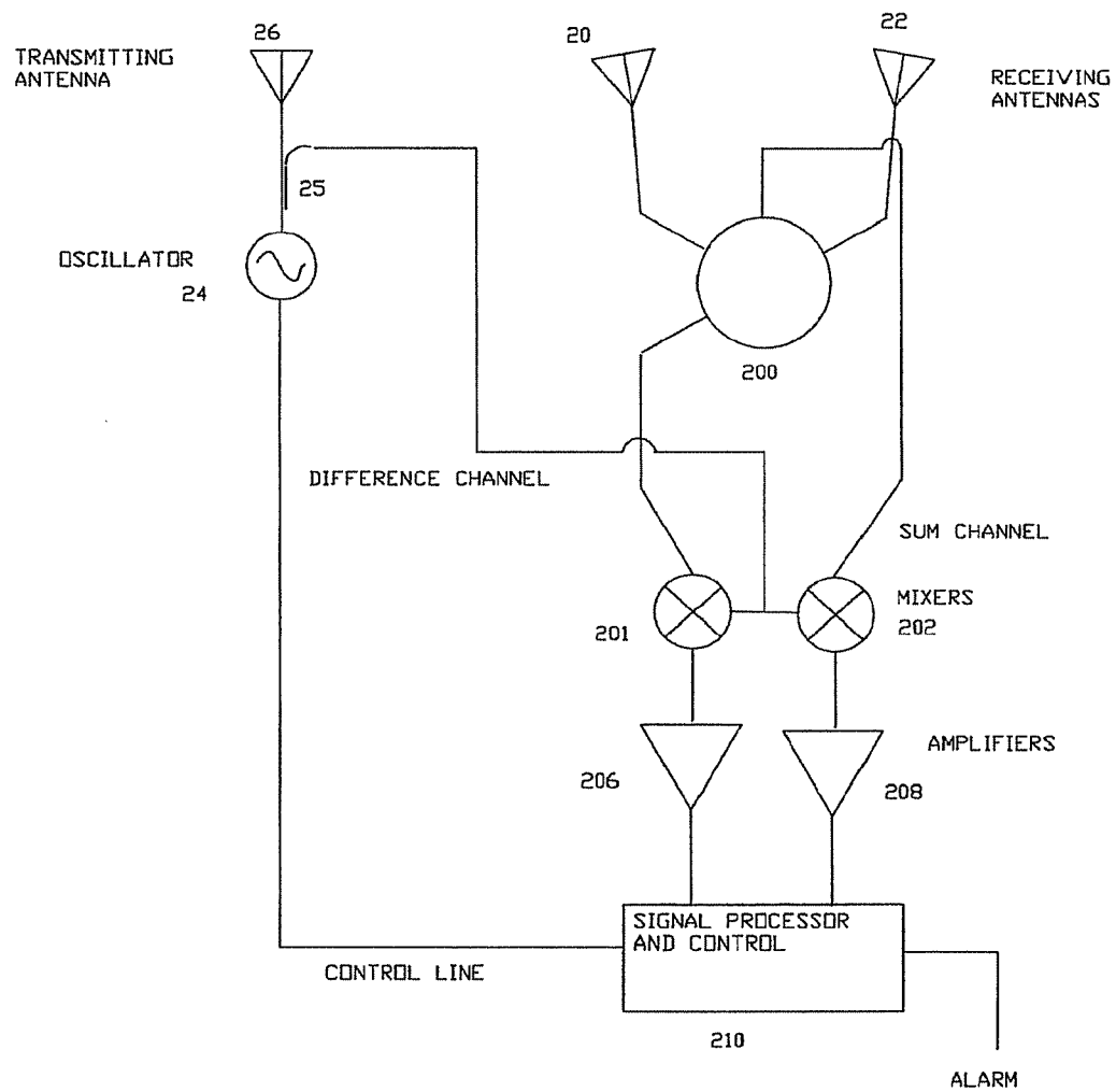
FIGURE 5 - AMPLITUDE MONOPULSE SENSOR
