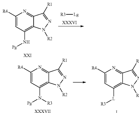
Scheme 13:
