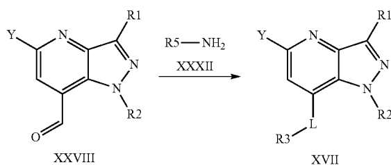
Scheme 11:
