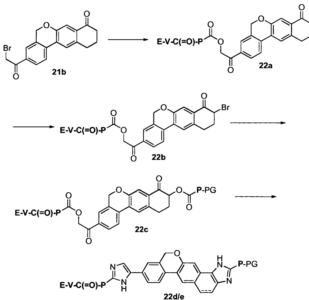
Scheme 22. Representative synthesis of E-V-C(=O)-P-W-P-R
