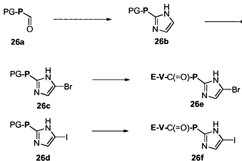
Scheme 26. Representative syntheses of E-V-C(=O)-P-R and R 1 -P-R
