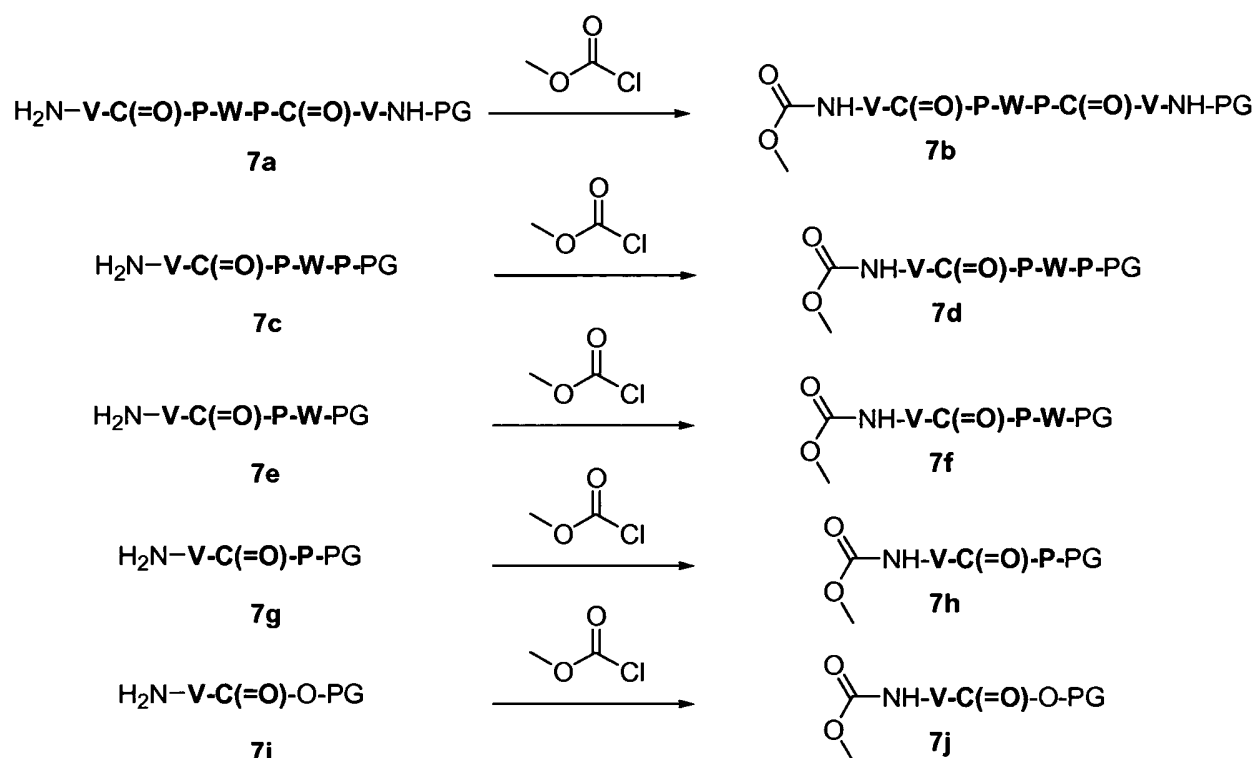
Scheme 7. Representative synthesis of E-V-C(=O)-R 1
