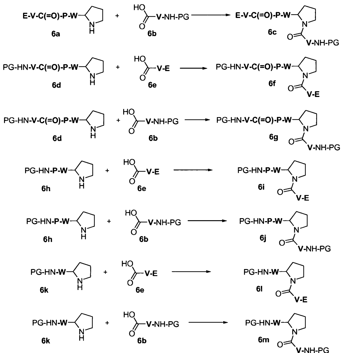
Scheme 6. Representative synthesis of R^1\text{-V-C(=O)-P-R}^2
