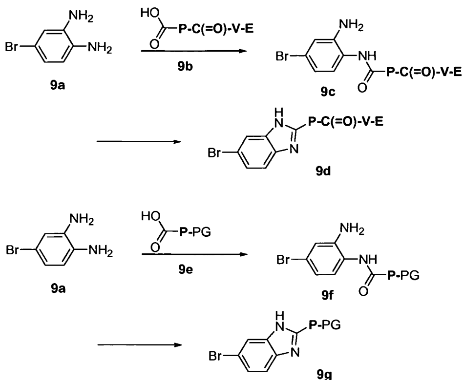
Scheme 9. Representative synthesis of R^1 -P- R^2
