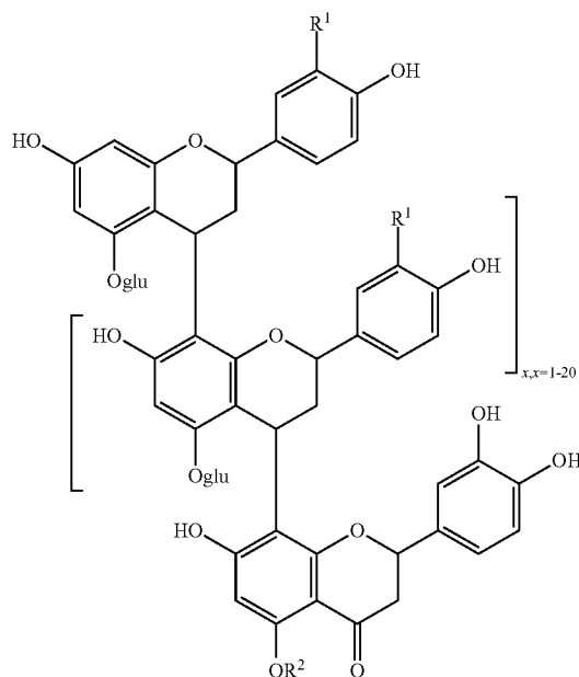
Scheme 3. Representative structures of a proanthocyanidin (PAs).
