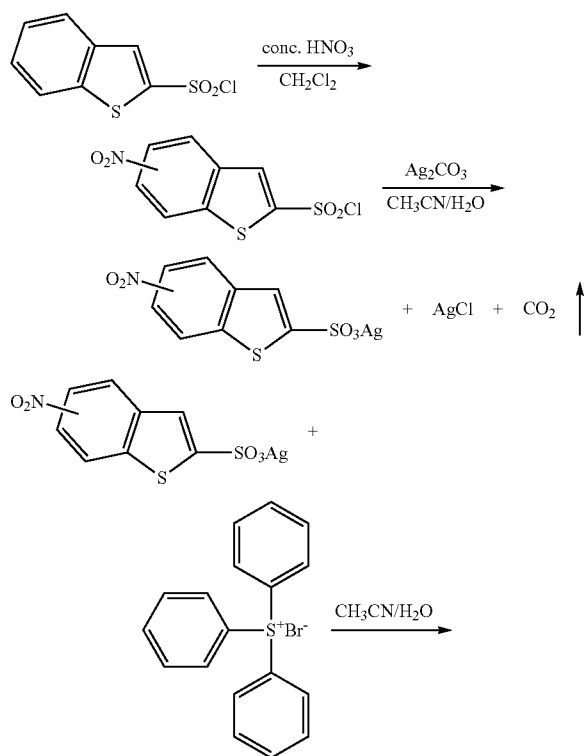
Scheme 1. Synthesis of fluorine-free fused-ring heteroaromatic PAGs.
