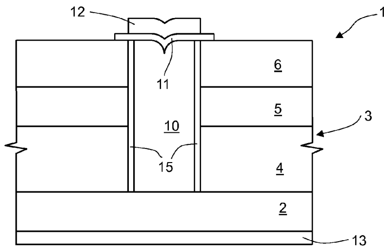
Fig. 1 Known Art
