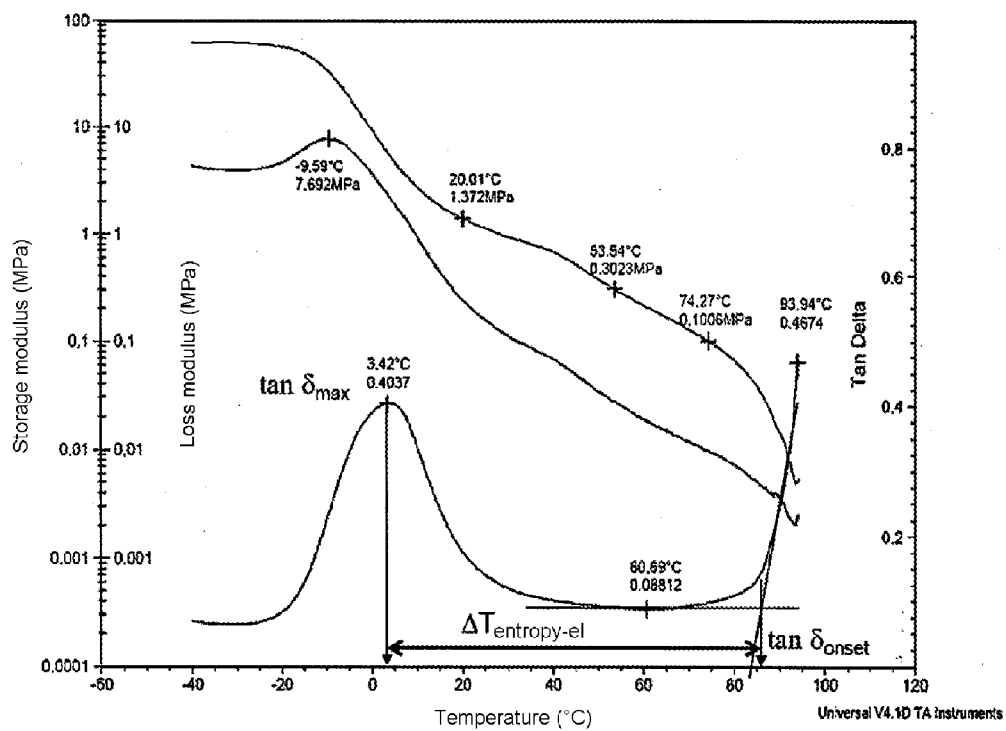
Figure 1: Determination of the temperature/application spectrum \Delta T_{\text{entropy-el}} from \tan \delta_{\text{max}} and \tan \delta_{\text{onset}} for melt adhesive 3
